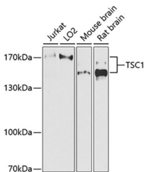
Fig. 1. Western blot analysis of extracts of various cell lines, using TSC1 antibody at 1:1000 dilution. Secondary antibody: HRP-labeled Goat Anti-Rabbit IgG(H+L) (A0208) at 1:1000 dilution. Lysates/proteins: 25 \mu g per lane. Blocking buffer: QuickBlock™ Blocking Buffer (P0231). Detection: BeyoECL Star (P0018A). Exposure time:1s.
