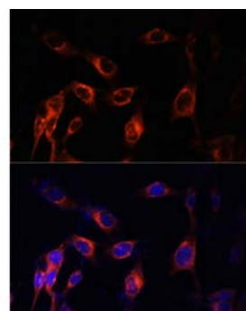
Fig. 2. Immunofluorescence analysis of NIH-3T3 cells using TSC1 Polyclonal Antibody at dilution of 1:100 (40x lens). Blue: DAPI for nuclear staining.
